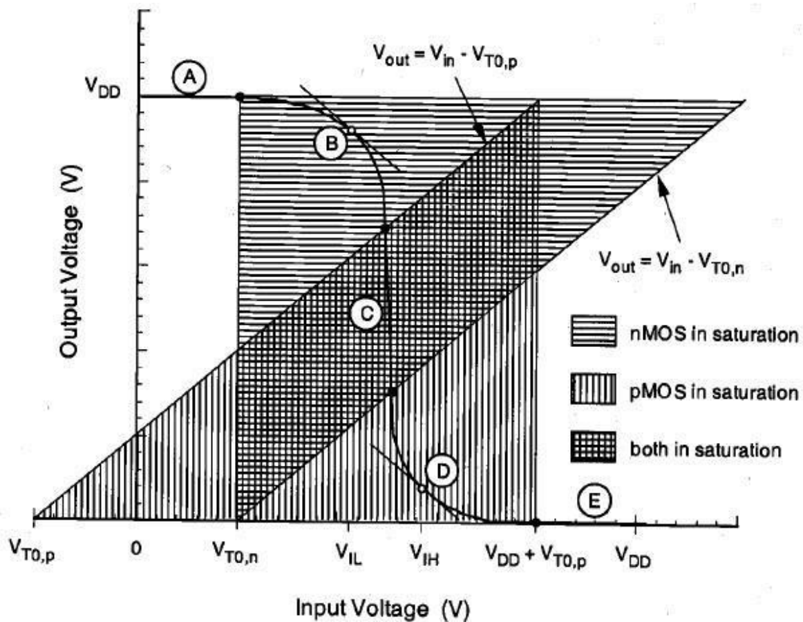
Fig-9 Operating regions of the CMOS inverter.
