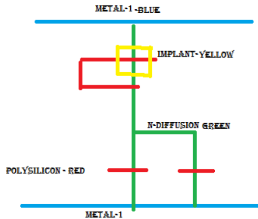
FIG.STICKDIAGRAMOFNORGATE.
