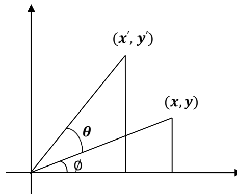
Fig. 3.2: - Rotation.
