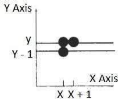
Fig. 6.4:-From position (x,y) on a scan line, the next position across the line has coordinates (x+1,y), and the position immediately below on the next line has coordinates (x,y-1).
