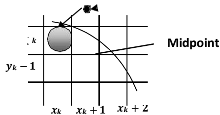
Fig. 2.10: - Midpoint between candidate pixel at sampling position x_k + 1 along circle path.
