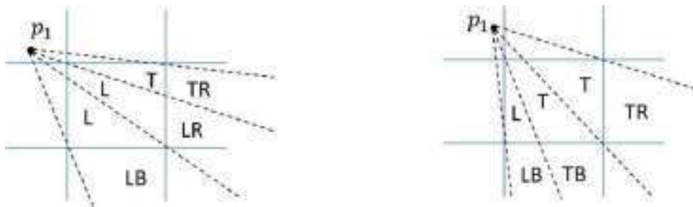
Fig. 3.10: - Two possible sets of clipping region when p1 is in corner region.
