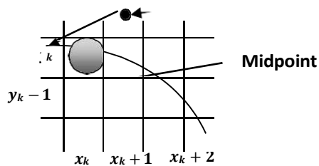
Fig. 2.15:- Midpoint between candidate pixels at sampling position x_k + 1 along an elliptical path.
