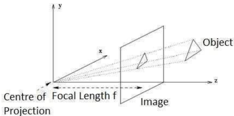
Fig. 4.2: - perspective projection
