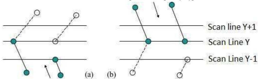
Fig. 2.18: - adjacent scan line intersects with polygon edge.
