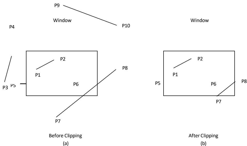
Fig. 3.5: - Line clipping against a rectangular window.
