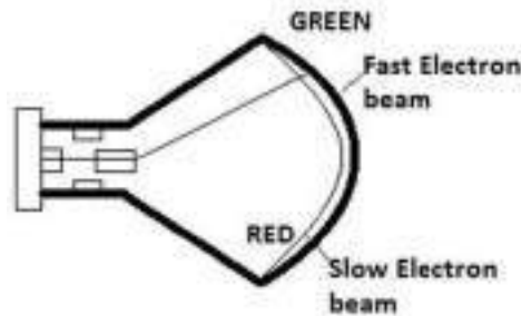
Fig. 1.5: - Beam-penetration CRT
