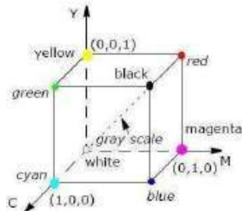
Fig. 6.14:- The CMY color model.
