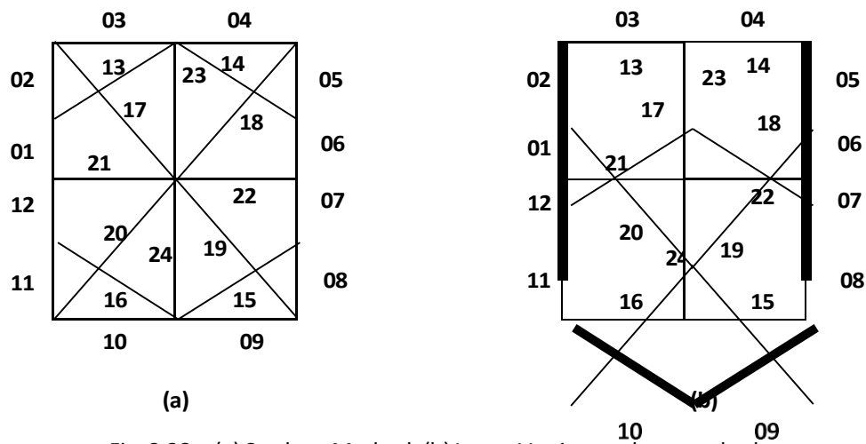
Fig. 2.28: - (a) Starbust Method. (b) Letter V using starbust method
