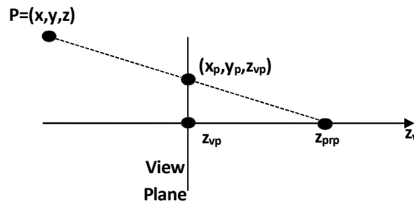
Fig. 5.19: - Perspective projection.
