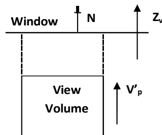
Fig. 5.22: - Shear operation in General parallel projection.
