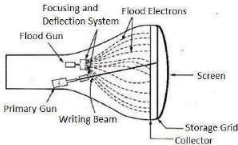
Fig. 1.7: - Direct-view storage tube.
