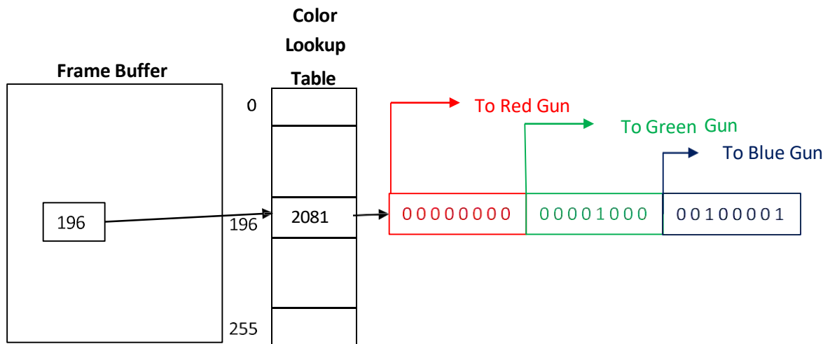
Fig. 2.35: - color lookup table.
