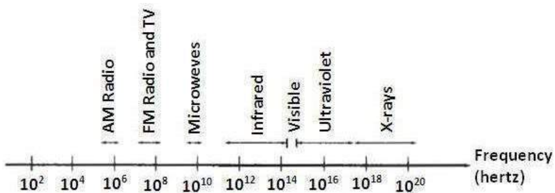
Fig. 6.11:- Electromagnetic spectrum.
