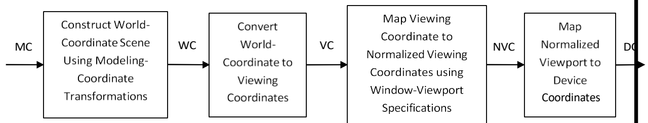
Fig. 3.2: - 2D viewing pipeline.
