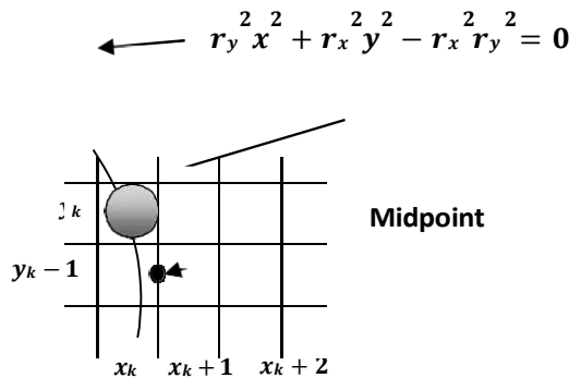
Fig. 2.16: - Midpoint between candidate pixels at sampling position y_k - 1 along an elliptical path.
