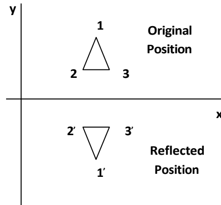
Fig. 3.9: - Reflection about x - axis.
