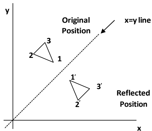
Fig. 3.12: - Reflection about x=y line.
