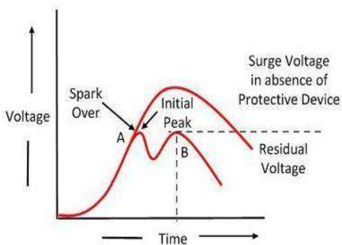
Voltage Characteristic
