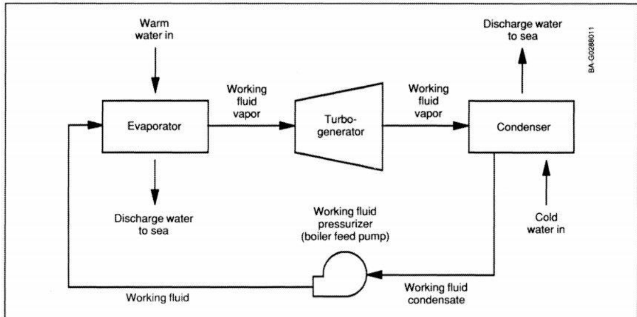
Closed cycle OTEC Plants
