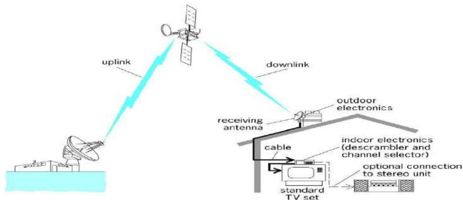
Direct broadcasting satellite system
