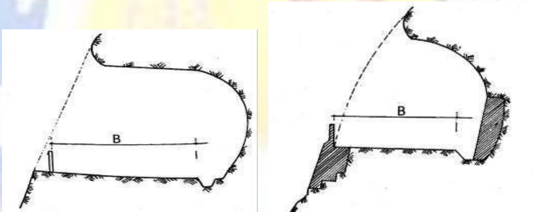
Fig: WithAccommodatingRoad-WayOnlyandWithRetainingandBreastWalls
