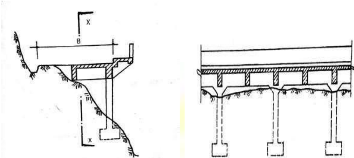
Fig: CrossSectionandL-Section(X-X)ofaSemi-Bridge.
