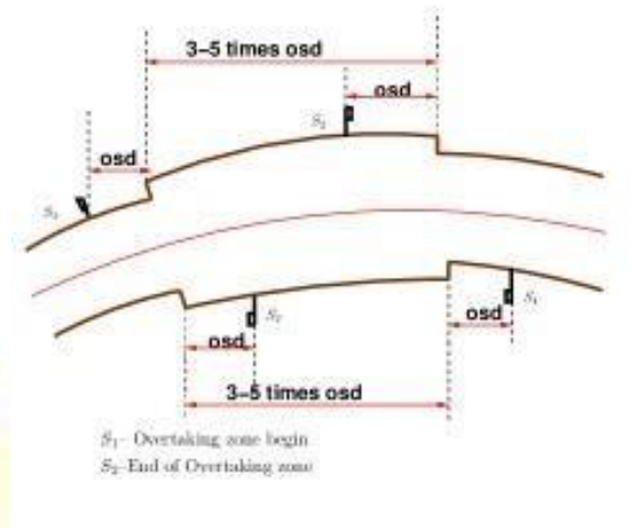
Figure: Overtaking zones
