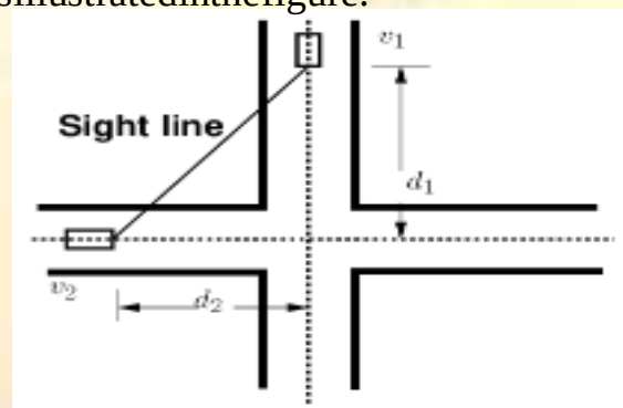
Figure: Sight distance at intersections
