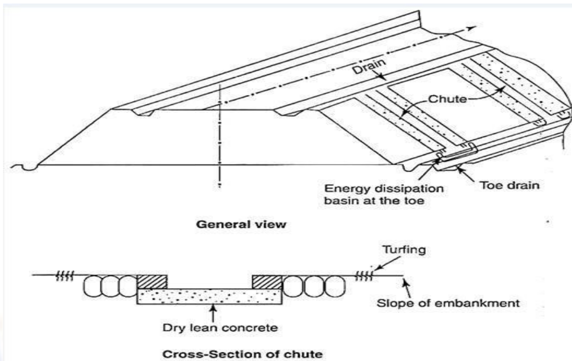
Fig.DrainagesystemforhighEmbankment
