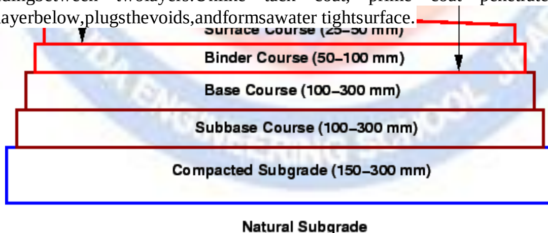
Figure 2: Typical cross-section of a flexible pavement
