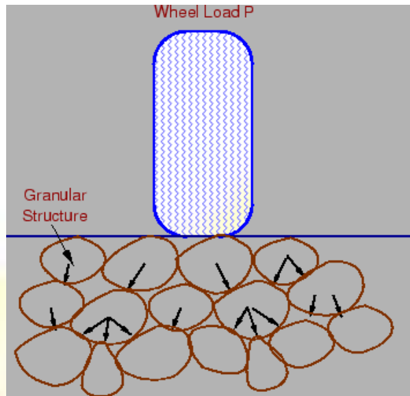
Figure1 :Loadtransferringgranularstructure
