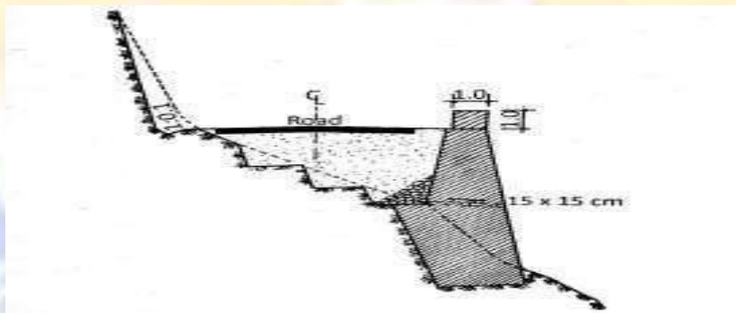
Typical Cross Section of Embankment with retaining walls
