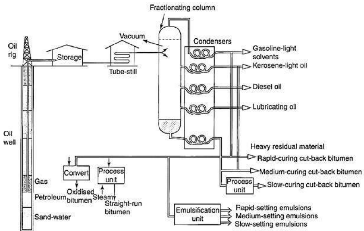
Fig. Schematic flowchart of petroleum refining
