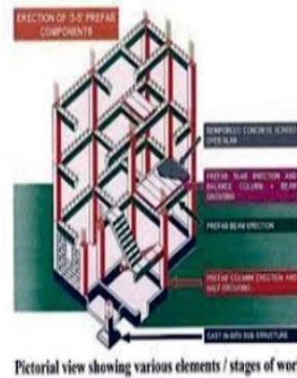
Figure 12: 3-S System
