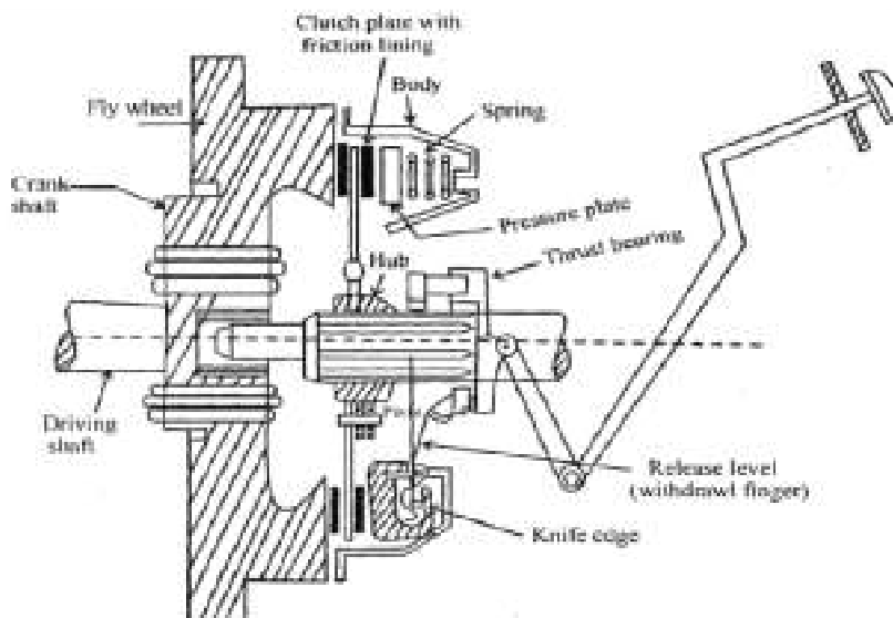
Fig. Single Plate Clutch
