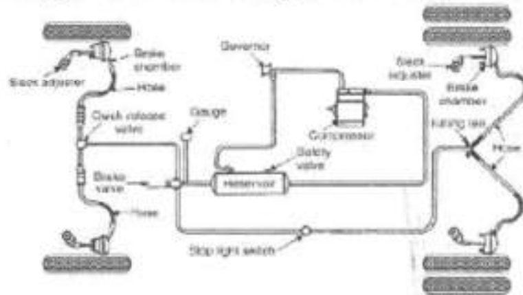
Layout of an air brake system for bus or truck.
