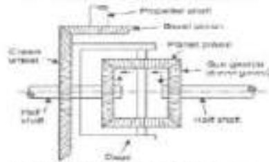
(a) Simple differential-simplified diagram
