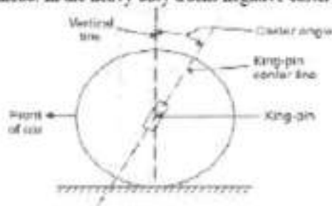
Caster angle (Positive)
