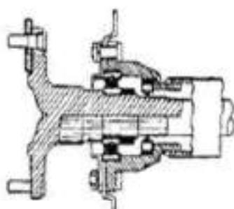
Fig. Semi-floating ball-race-bearing.
