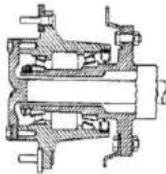
Fig. Fully floating axle.
