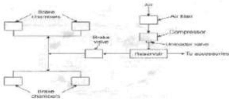
General arrangement of an air brake system.
