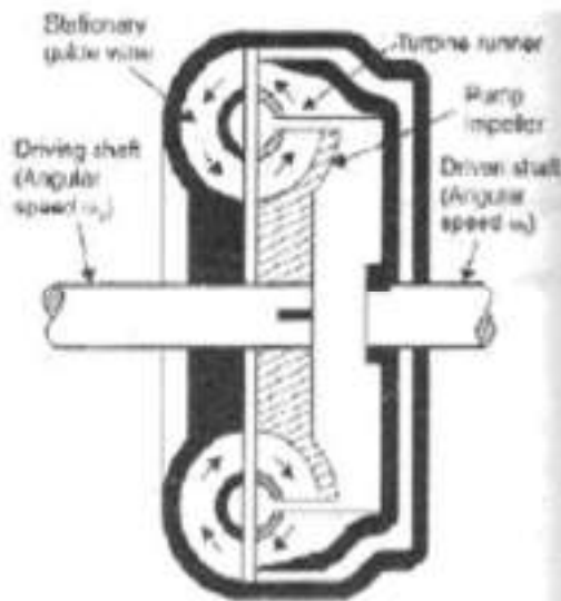
Hydraulic torque converter
