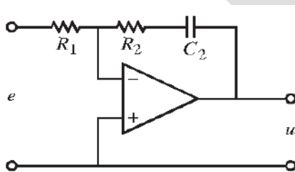
(a) PI controller
